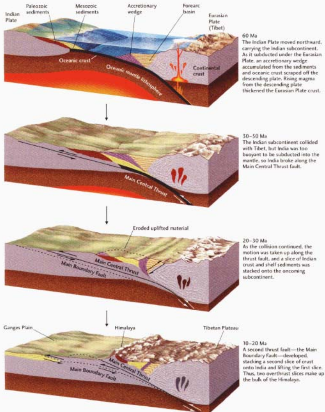
Figure 10.15 Cross sections showing the sequence of events that have caused the Himalayan orogeny, simplified and vertically
